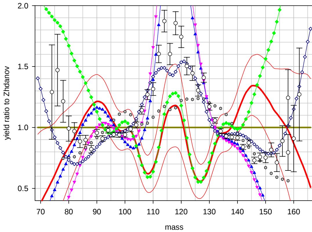
Benchmark A: ^{238}\text{U} around 13 MeV, post neutron emission yield ratios to Zhdanov's data lower graph: partial plot (high and low values omitted), for legend see upper graph.
